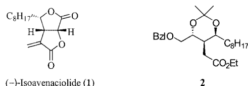
Scheme 1. Structures of (–)-isoavenaciolide ( 1 ) and advanced precursor 2
