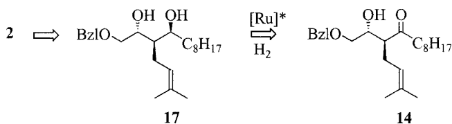
Scheme 4. New pathway to compound 2 by asymmetric hydrogenation of β-hydroxy ketone 14
