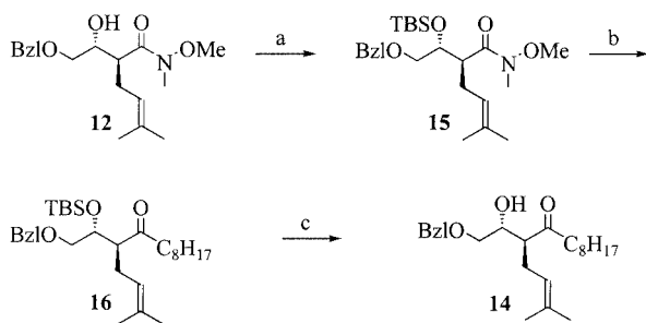
Scheme 6. Reagents and conditions: (a) 2,6-lutidine, TBSOTf, CH 2 Cl 2 , 0 °C, 1 h, 99%; (b) n C 8 H 17 Li (2 equiv.), THF, -50 °C, 2 h, 73%; (c) n Bu 4 NF, THF, 0 °C, 2 h, 96%
