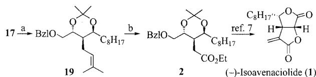
Scheme 8. Reagents and conditions: (a) 2,2-dimethoxypropane, acetone, PPTS cat., room temp., 20 min, 98%; (b) O 3 , 2.5 M ethanolic NaOH, CH 2 Cl 2 , –78 °C, 1 h, 88%
