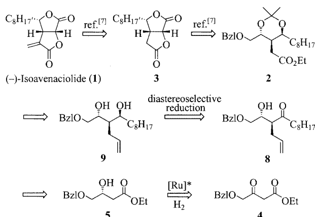
Scheme 2. Retrosynthetic analysis for (–)-isoavenaciolide ( 1 )
