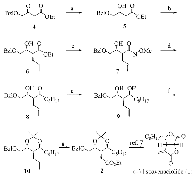
Scheme 3. Reagents and conditions: (a) 0.03 mol % [(S)-(MeO-BIPHEP)RuBr 2 ], H 2 (10 bar), EtOH, 80 °C, 48 h, 94%, e.e. = 98%; (b) LDA (2 equiv.), THF, –78 °C, 1 h; allyl bromide (2.5 equiv.), HMPA (1.2 equiv.), –78 °C for 1 h then –20 °C for 1 h, 81%, d.e. = 97%; (c) MeNHOMe·HCl (4.7 equiv.), i PrMgCl (9 equiv.), THF, –20 °C, 80%; (d) n C 8 H 17 Li (2.3 equiv.), Et 2 O/THF, –10 °C, 5 h, 85%; (e) Me 4 NHB(OAc) 3 (6 equiv.), CH 3 CN/AcOH (1:1), –20 °C, 21 h, 94%, d.e. = 80%; (f) 2,2-dimethoxypropane, acetone, PTSA cat., room temp., 1 h, 94%; (g) O 3 , 2.5 M ethanolic NaOH, CH 2 Cl 2 , –78 °C, 3 h, 80%
