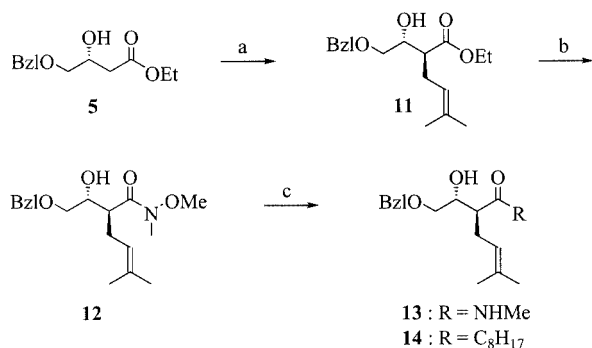
Scheme 5. Reagents and conditions: (a) LDA (2.5 equiv.), THF, -78 °C, 1 h; 4-bromo-2-methylbut-2-ene (2.5 equiv.), HMPA (1.2 equiv.), -78 °C for 3 h then -20 °C for 1 h, 78%, d.e. = 99%; (b) MeNHOMe·HCl (3 equiv.), n BuLi (6 equiv.), THF, -78 °C, 2 h, 92%; (c) n C 8 H 17 Li (2.7 to 4 equiv.), THF or Et 2 O, -40 °C, 3 h, 36–63% of 13 and 5–24% of 14
